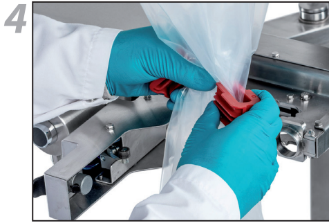
Insert film into the crimp
